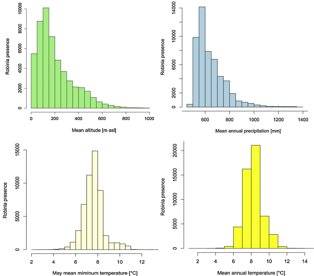
Fig. 2. Frequency distribution of Robinia along altitudinal, rainfall and temperature gradients. Environmental variables were derived from WorldClim ( http://www.worldclim.org ). Sources of the data on the distribution of Robinia are cited in Chapter 3 (current distribution). Austria and Switzerland were excluded from the analysis due to the low precision of the occurrence data for these countries.
